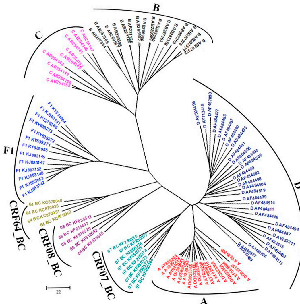
Fig. 1. Unrooted neighbor-joining tree depicting the genetic relationship among the 102 complete genomes including 8 subtypes and CRFs by SNV method. Each group is highlighted with a different color.
