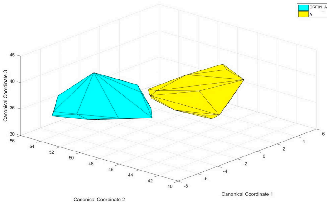
Fig. 6. Three dimensional projection for 236 CRF01_AE and 95 A complete genomes. The cyan and yellow convex polygon are formed by CRF01_AE and A viruses respectively. The two subtypes are clearly separate from each other. (For interpretation of the references to color in this figure legend, the reader is referred to the web version of this article.)
