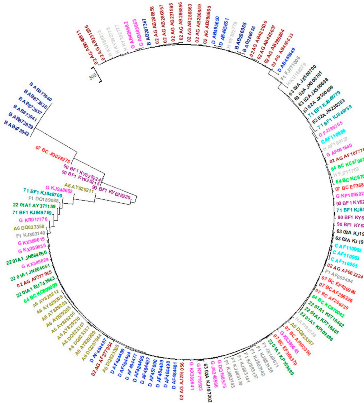
Fig. 4. Phylogenetic tree depicting the genetic relationship among the 130 pol genes including 14 subtypes and CRFs by NV method. Each group is highlighted with a different color.
