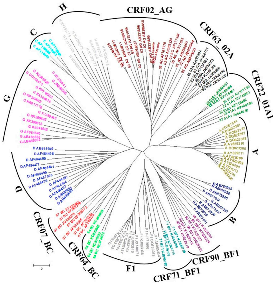
Fig. 2. Unrooted neighbor-joining tree depicting the genetic relationship among the 130 pol genes including 14 subtypes and CRFs by SNV method. Each group is highlighted with a different color.
