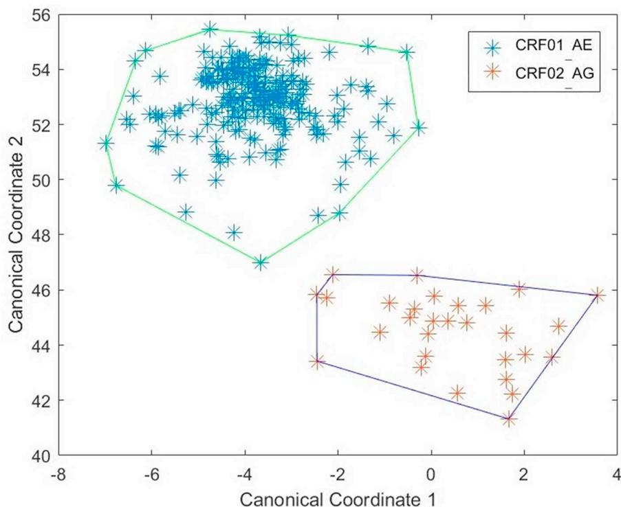
Fig. 5. Two dimensional projection for 236 CRF01_AE and 29 CRF02_AG complete genomes. The blue and orange convex polygon are formed by CRF01_AE and CRF02_AG viruses respectively. The two subtypes are clearly separate from each other. (For interpretation of the references to color in this figure legend, the reader is referred to the web version of this article.)
