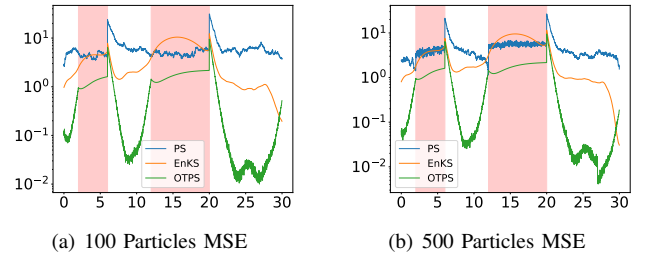
Fig. 4. The MSE of three different smoother algorithms are shown. There is no observation in time periods marked in red. The dimension of the state and observation is n = m = 10 .
