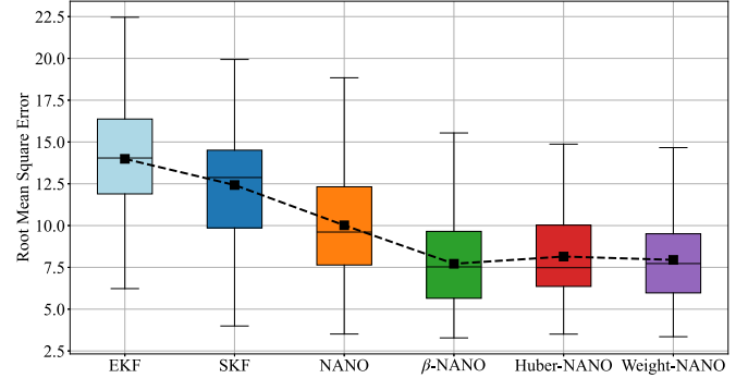
Fig. 3. Box plot of RMSE for EKF, SKF and NANO filter and its robust variants on the 6D coupled Lorenz system with contaminated measurements.
