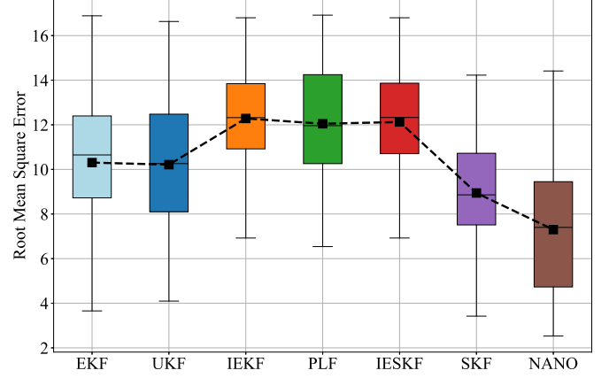
Fig. 2. Box plot of RMSE for EKF, UKF, IEKF, PLF, IESKF, SKF and NANO filter on the 6D coupled Lorenz system over 200 Monte Carlo runs. Note that the black square “■” represents the average RMSE over all the Monte Carlo experiments.
